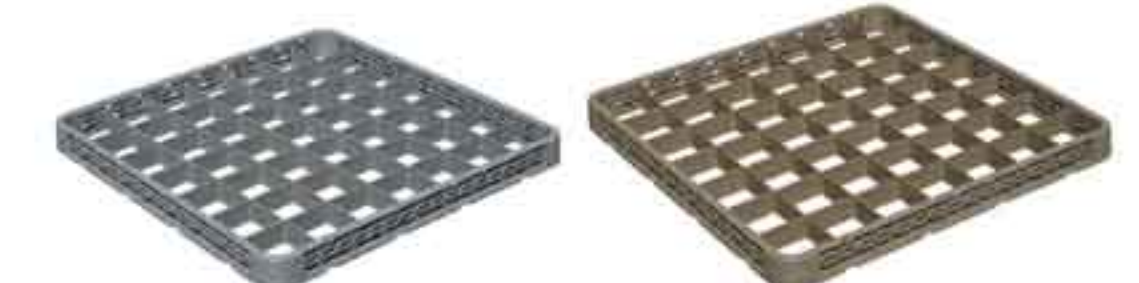
49 Compartment Dropped Extender GR0911012 L500xW500xH45mm
